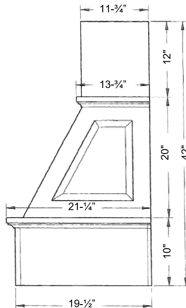
Side – Wall Hood
