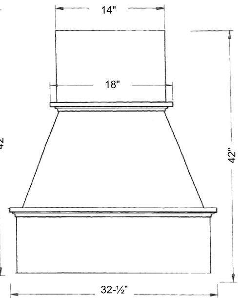
Side - Island Hood
